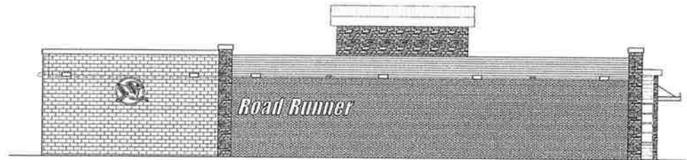
② BACK ELEVATION SCALE: 3/16" = 1'-0"
