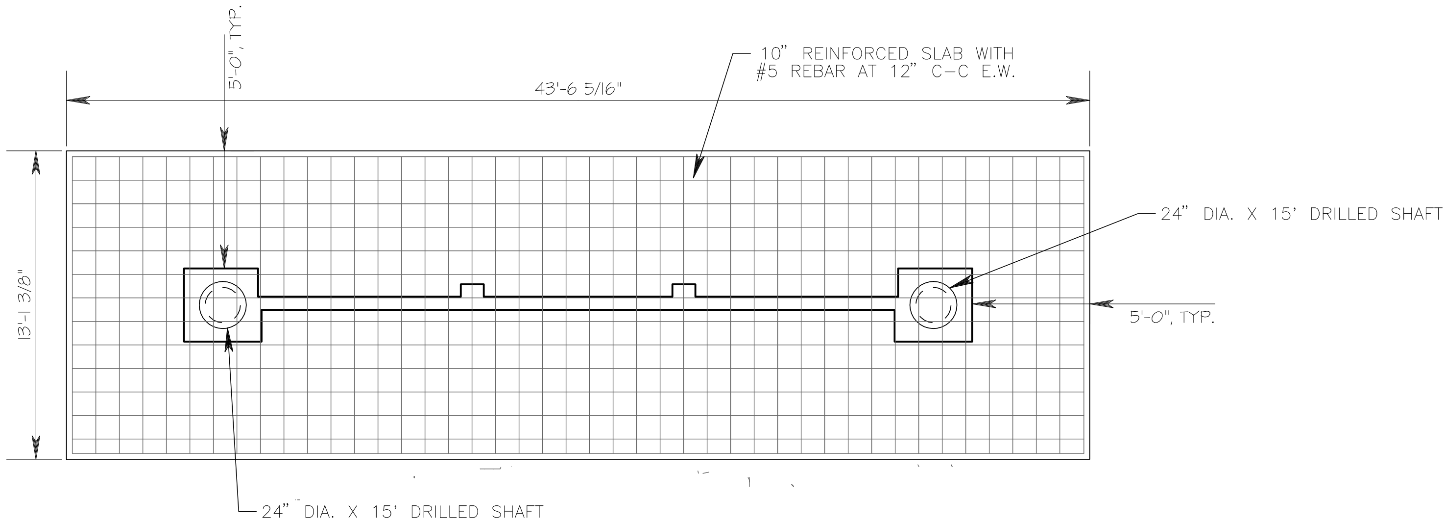
FOUNDATION PLAN
