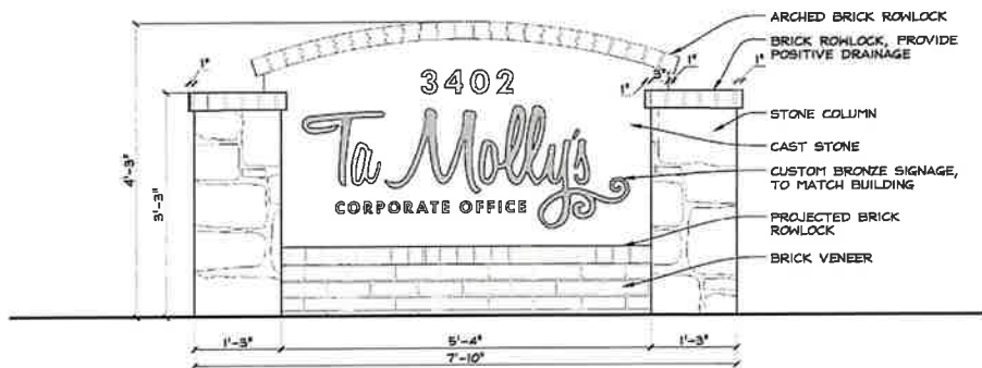
ELEVATION @ MONUMENT SIGN
