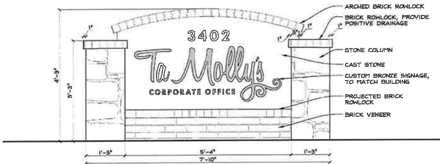
ELEVATION of MONUMENT SIGN
