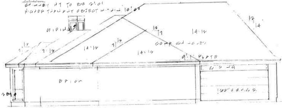
LEFT ELEVATION OVERALL 14'0"
