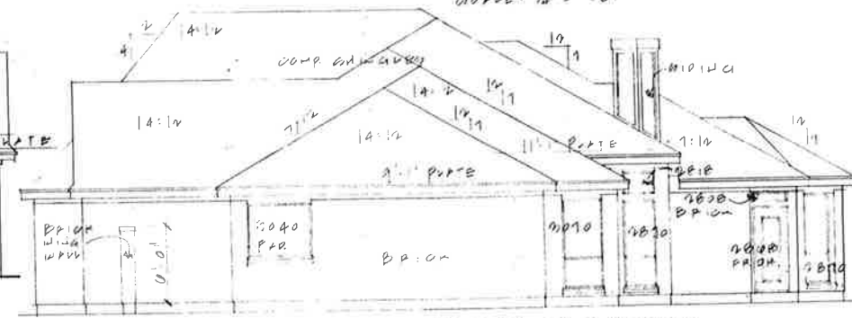
RIGHT ELEVATION OVERALL 14'0"
