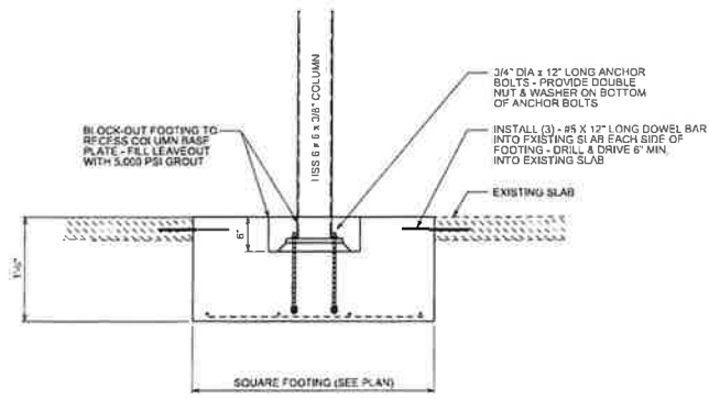
SECTION A SECTION THRU NEW HSS COLUMN FOOTING SCALE: 3/4"=1'-0"
