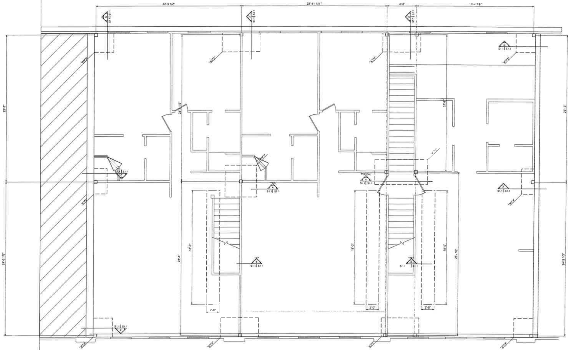
FOUNDATION PLAN
