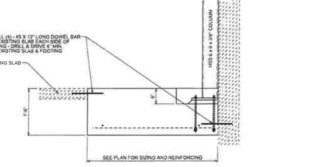
SECTION C SECTION THRU FOOTING @ PERIMETER WALLS SCALE: 3/4"=1'-0"
