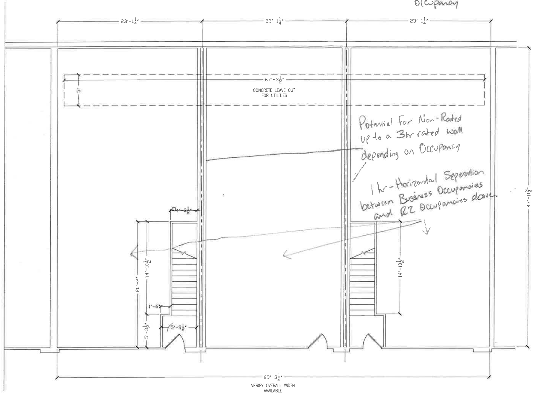
Proposed Comm. Space Scale 1/4" = 1'-0"
