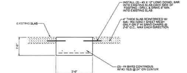
SECTION B TYPICAL SECTION @ INTERIOR LOAD BEARING WALL SCALE: 3/4"=1'-0"
