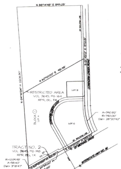
DETAIL - TRACT NO. 2 AND RESTRICTED AREA
